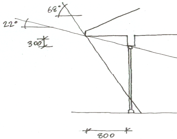
A glazed door with an eave 300mm above the head of the door needs an eave of about 800mm
