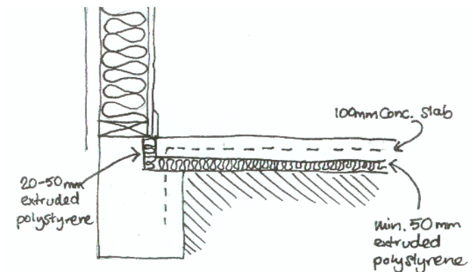
A method of insulating a slab edge
