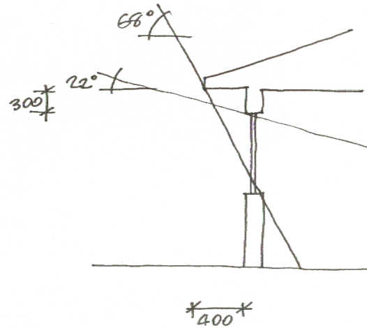
A window with a sill height of 1000mm needs an eave of around 400mm
