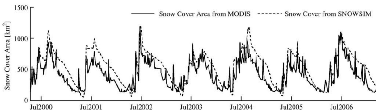
Figure 5: Time series of MODIS-derived snow-covered area in the Pukaki catchment compared to snow-cover predicted from the SNOWSIM model. Source: Sirguey et al (2009) – their figure 15.
