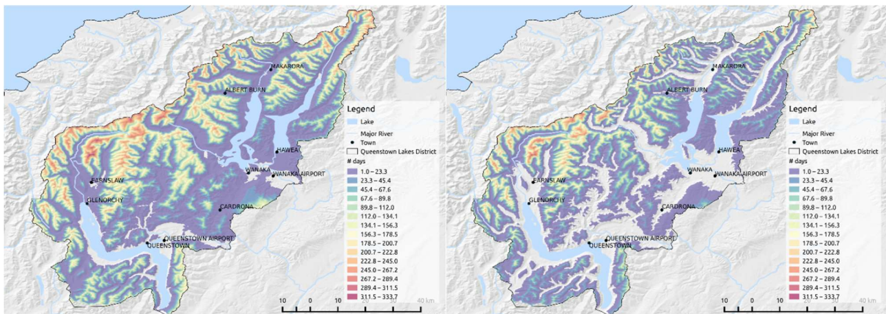
Figure 37: Average snow-cover duration (days) for the District for the base-period (2000-2009, left), and for the end of the century (2090-2099, right) under RCP8.5.
