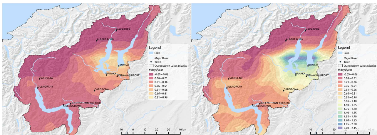
Figure 32: Change in the number of low RH days for the mid-century period (2040-49, left) and the last decade of the century (2090-2099, right) for the RCP8.5 emissions scenario. Note the change in colour-scale between the two panels.
