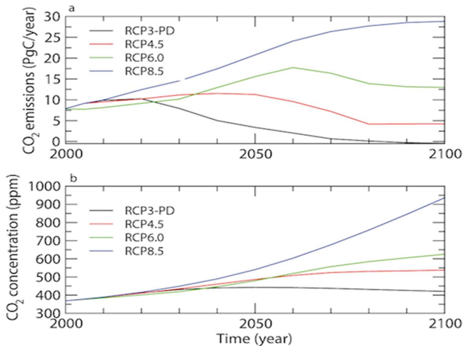
Figure A1: \text{CO}_2 emissions and resultant atmospheric \text{CO}_2 concentrations for the four RCP scenarios. Note that in this figure RCP2.6 is listed as RCP3-PD i.e., the radiative forcing peaks at 3 \text{Wm}^{-2} in mid-century before declining to 2.6 \text{Wm}^{-2} in 2100 (IPCC, 2014).
