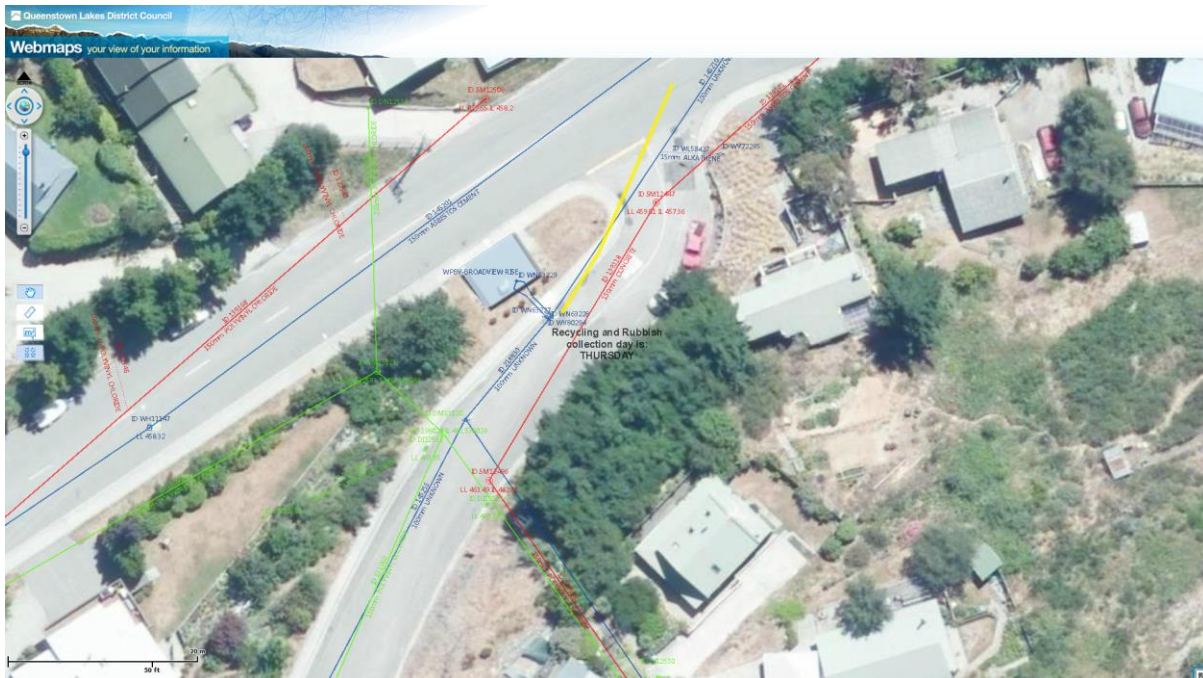
Figure 1 –Water Pump Station shown in Blue. Source – QLDC Website 09.03.15
