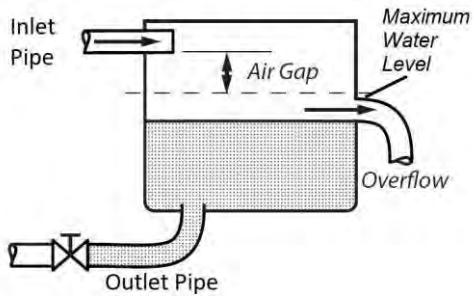
Figure 2-2 Air gap with overflow
