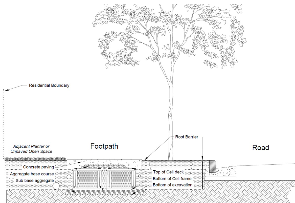
Drawing 2 - Partially engineered example – Directing roots underneath pavements (Image created by Arborlab, amended from DeepRoot drawing)
