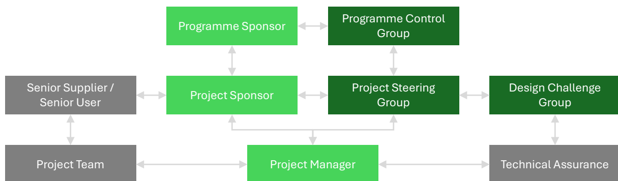
Figure 10: Project structure
